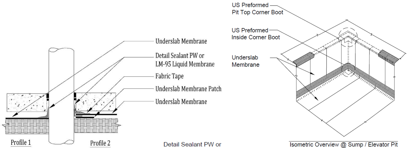
Section @ Underslab Membrane Penetration Detail
