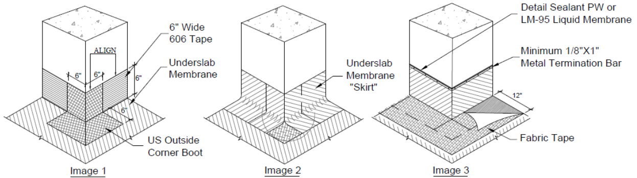
Preformed US Outside Corner Boot at a Corner or Column
